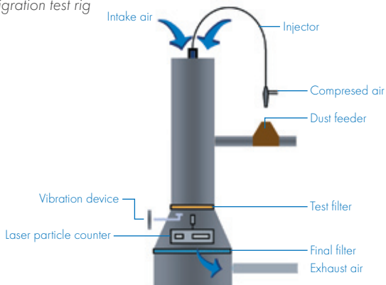
Migration test rig
