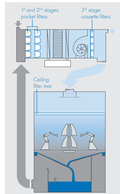
Painting system in air recirculation mode with 3 air recirculation stages and ceiling filter
